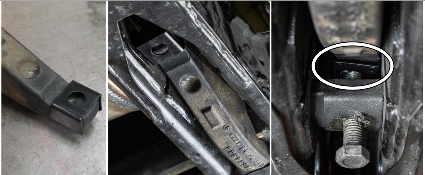
Figure 69: Cognito Torsion Key Retainer
