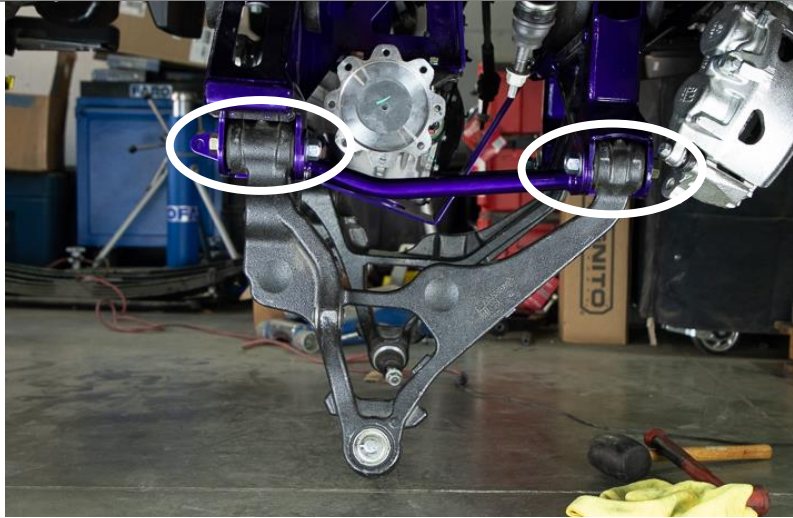
Figure 72: Lower Control Arm Bolts that do NOT get torqued at this step
