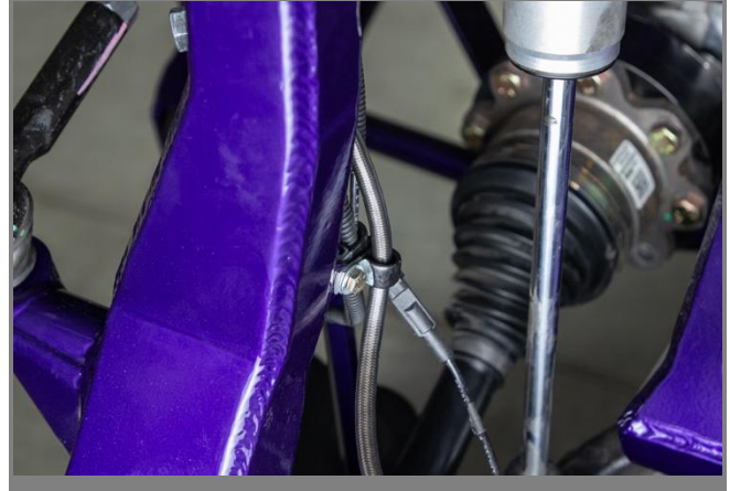
Figure 61: Driver Side Middle Spindle Tab & P-clamps
