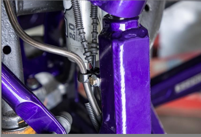
Figure 60: Driver Side Top Spindle Tab & P-clamps
