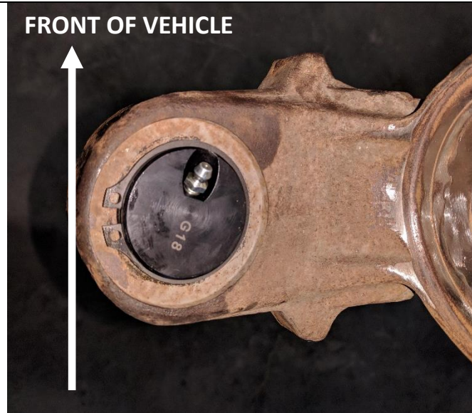
Figure 10. Lower Ball Joint Orientation
