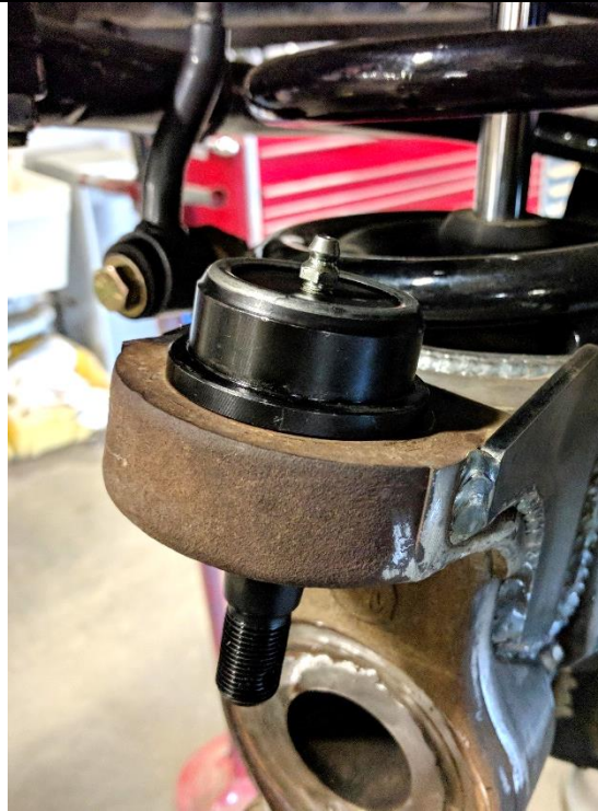
Figure 12. Upper Ball Joint Pressed In
