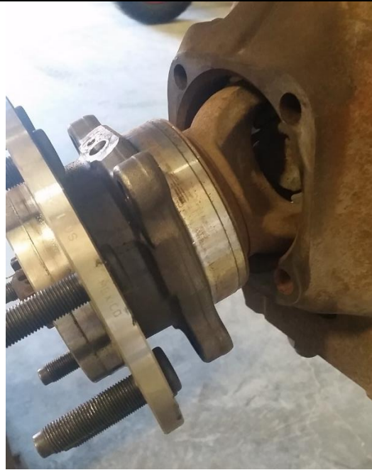
Figure 6. Removing Unit Bearing/Hub and Axle Assembly from Axle
